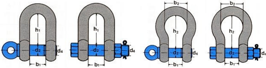
Chain Shackle with Screw collar pin (Type IV, B, Class 2)
